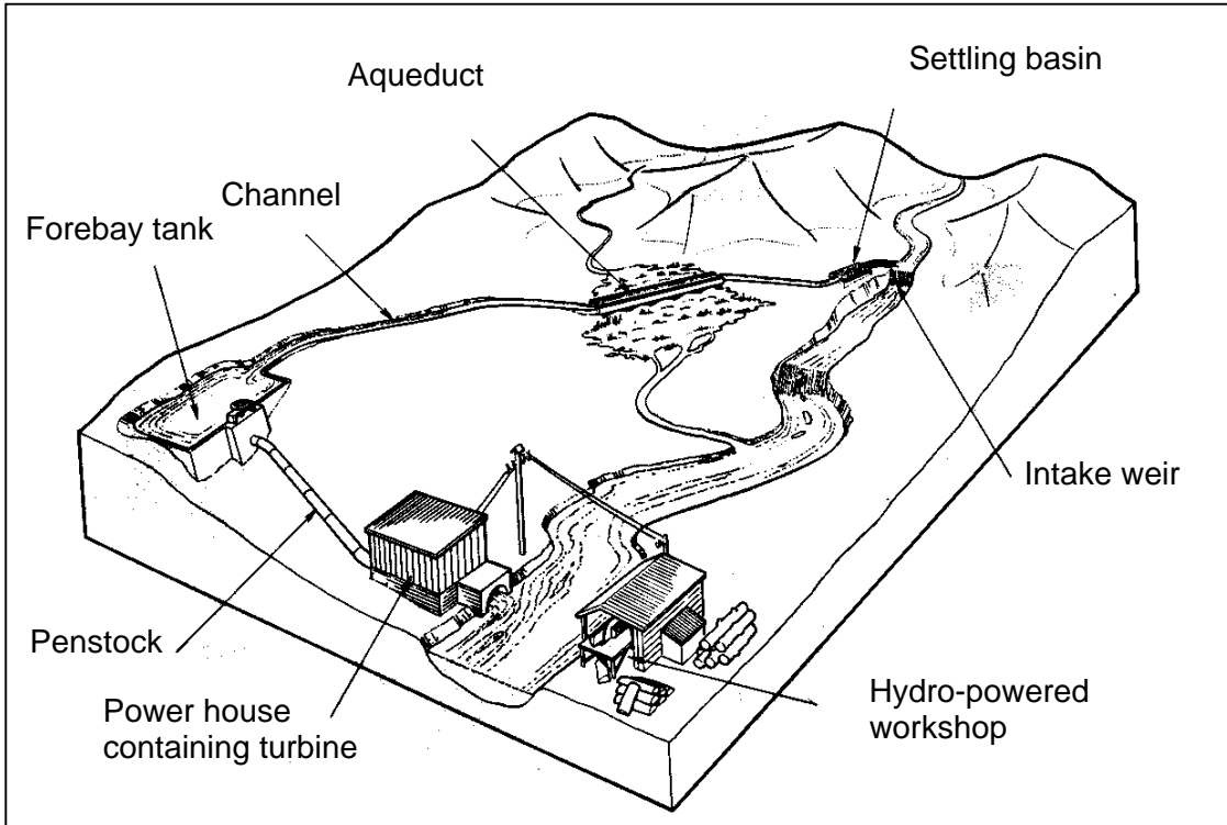
Figure 1: Layout of a typical micro hydro scheme
