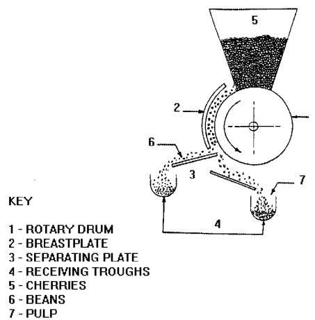
Figure 3: Separation of pulp and beans
