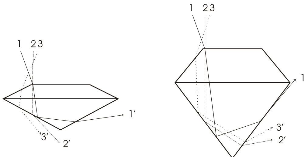
Figure 36: Paths of light in wrong cut stones.
